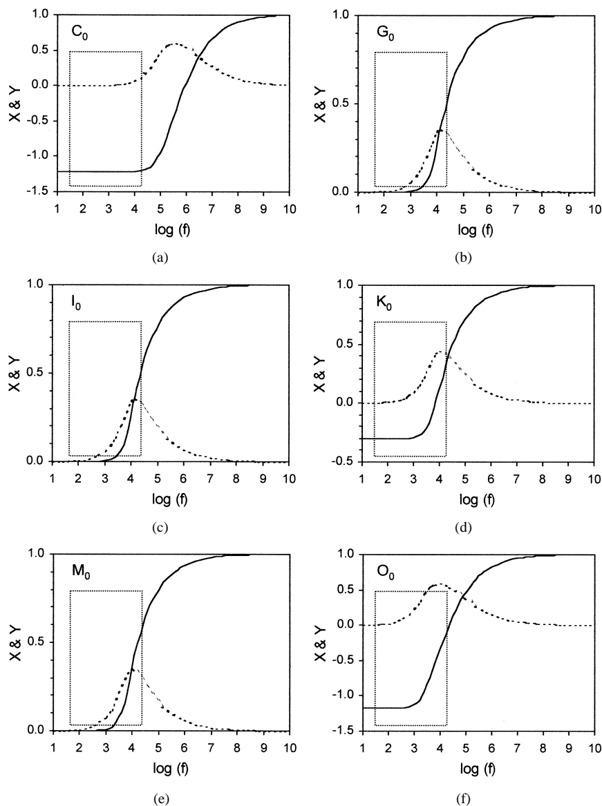
Fig. 5. Normalized EMIS spectra of six mine simulants, located at 10 cm from the GEM-3, using equivalent spheres as shown in Table I. Rectangles indicate the current GEM-3 bandwidth.
