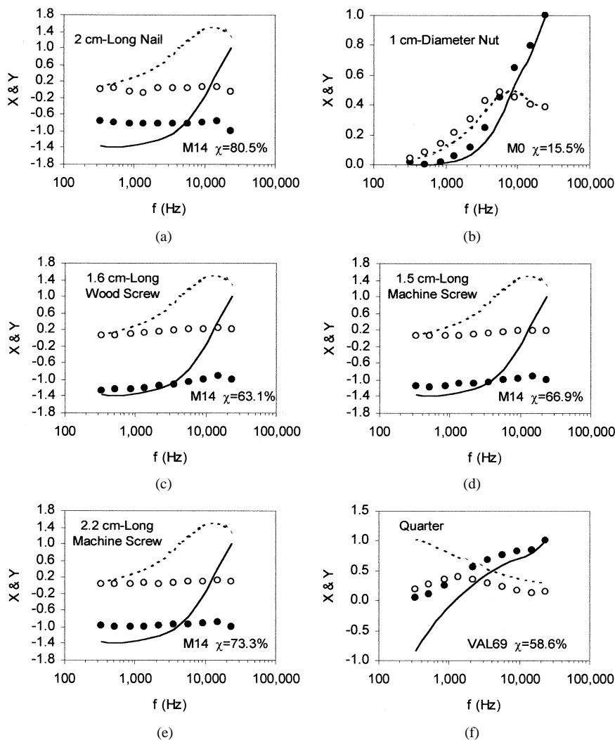
Fig. 9. Normalized spectra of selected clutter items (circles), along with the best matching library spectra (lines) shown in Figs. 7 and 8. It is obvious that majority of the clutter can be correctly rejected.
