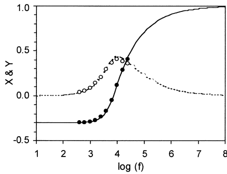
Fig. 3. Measured spectrum (circles) of a mine simulant K_0 is fit to the computed normalized spectrum (lines) to determine conductivity and permeability of an equivalent sphere. The solid circles stand for in-phase, and open circles for quadrature (same for the remaining figures).
