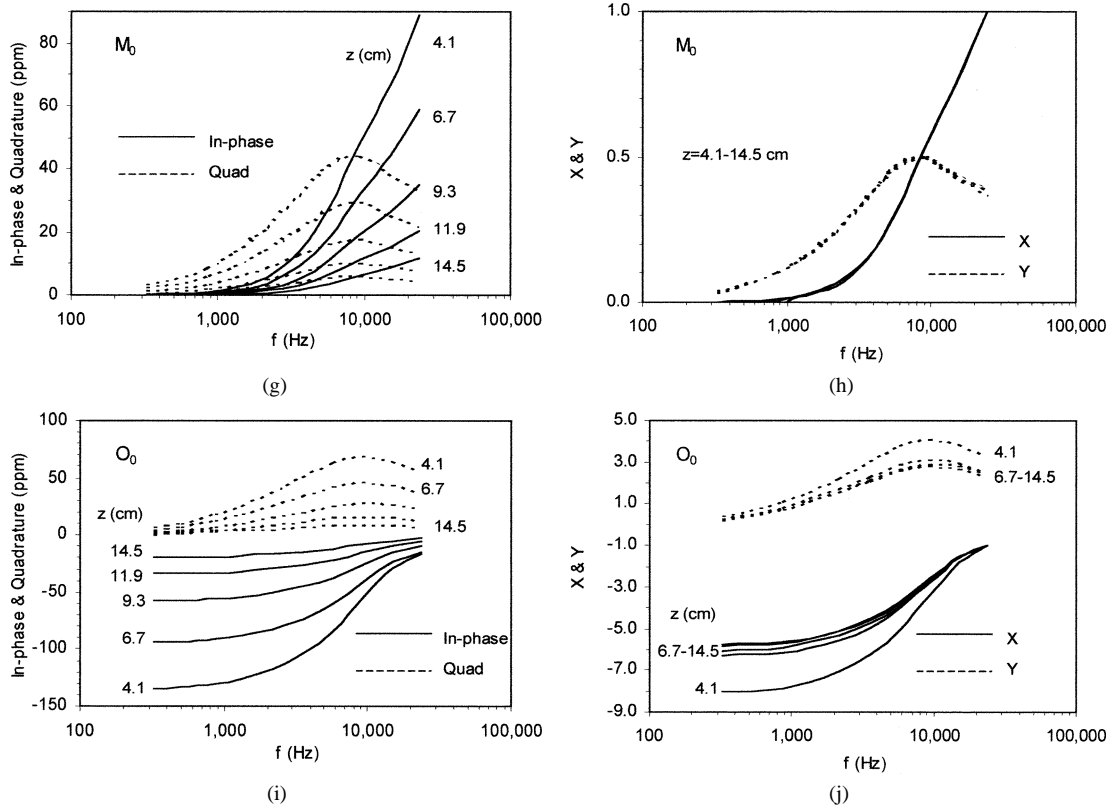
Fig. 6. (Continued) Measured EMIS spectra (left) for five mine simulants G_0 , I_0 , K_0 , M_0 , and O_0 located at varying distances to the GEM-3 sensor and their corresponding normalized EMIS spectra (right).
