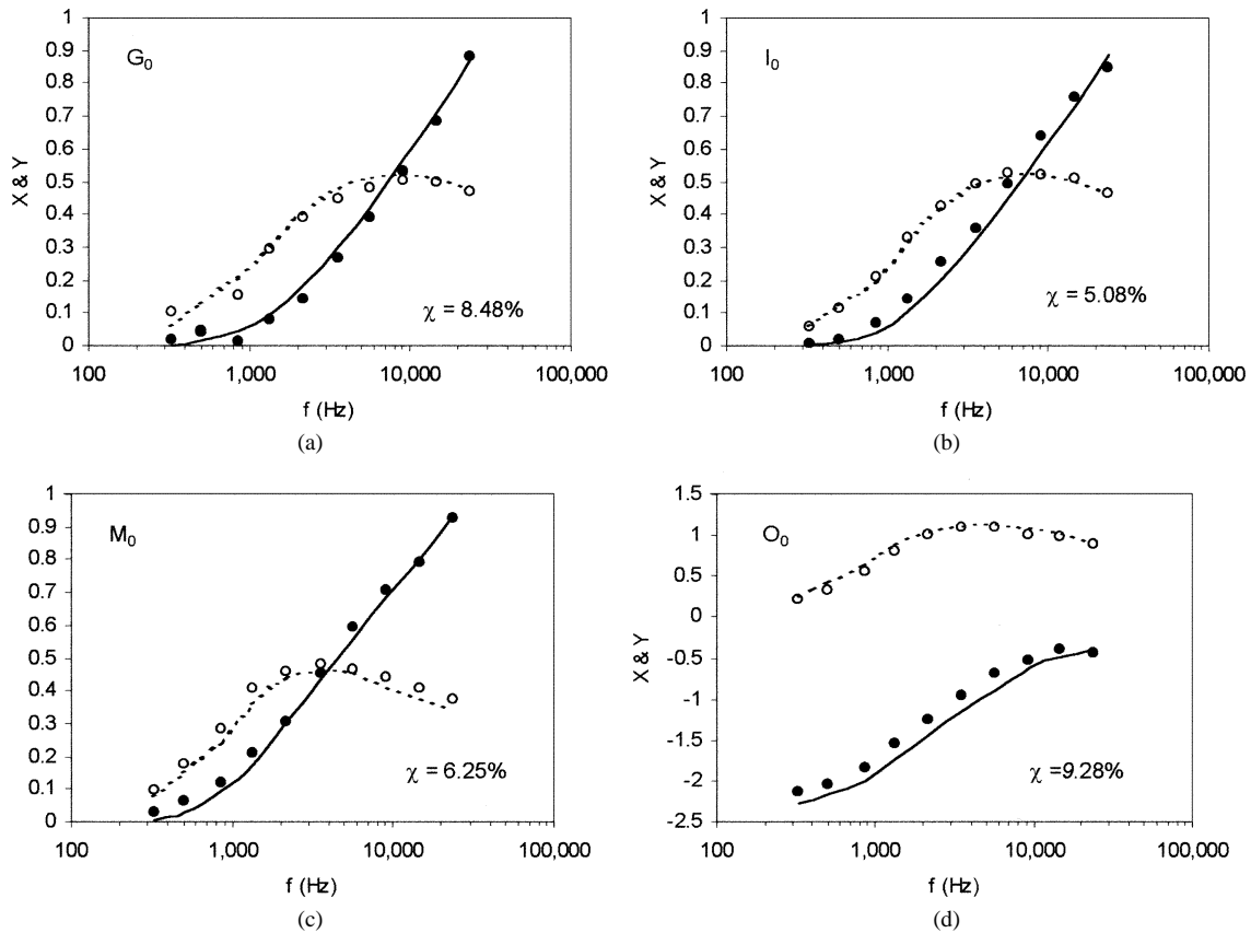
Fig. 7. Measured and normalized EMIS spectra (circles) of four mine simulants G_0 , I_0 , M_0 , and O_0 buried in a hard clay ground, along with the best matching library spectra (lines) all of which are correctly identified.
