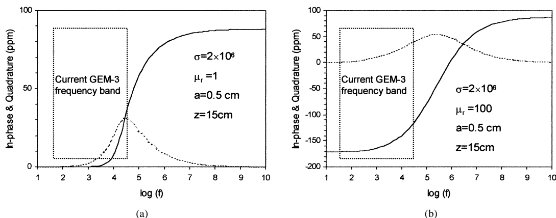
Fig. 2. Computed EMIS spectra of (a) nonpermeable and (b) permeable spheres with conductivity, relative permeability, radius, and depth as indicated. The rectangles show the current GEM-3 bandwidth. The solid lines stand for the in-phase, and the dotted lines for the quadrature (same for the remaining figures).
