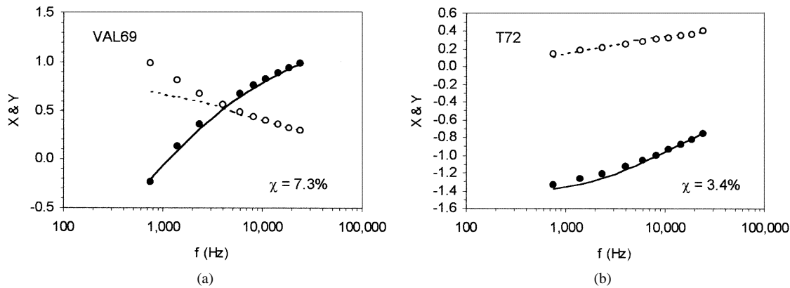
Fig. 11. Normalized EMIS spectra (circles) obtained from two blind grids at U.S. Army Test Site, along with the best matching library landmine spectra (lines).
