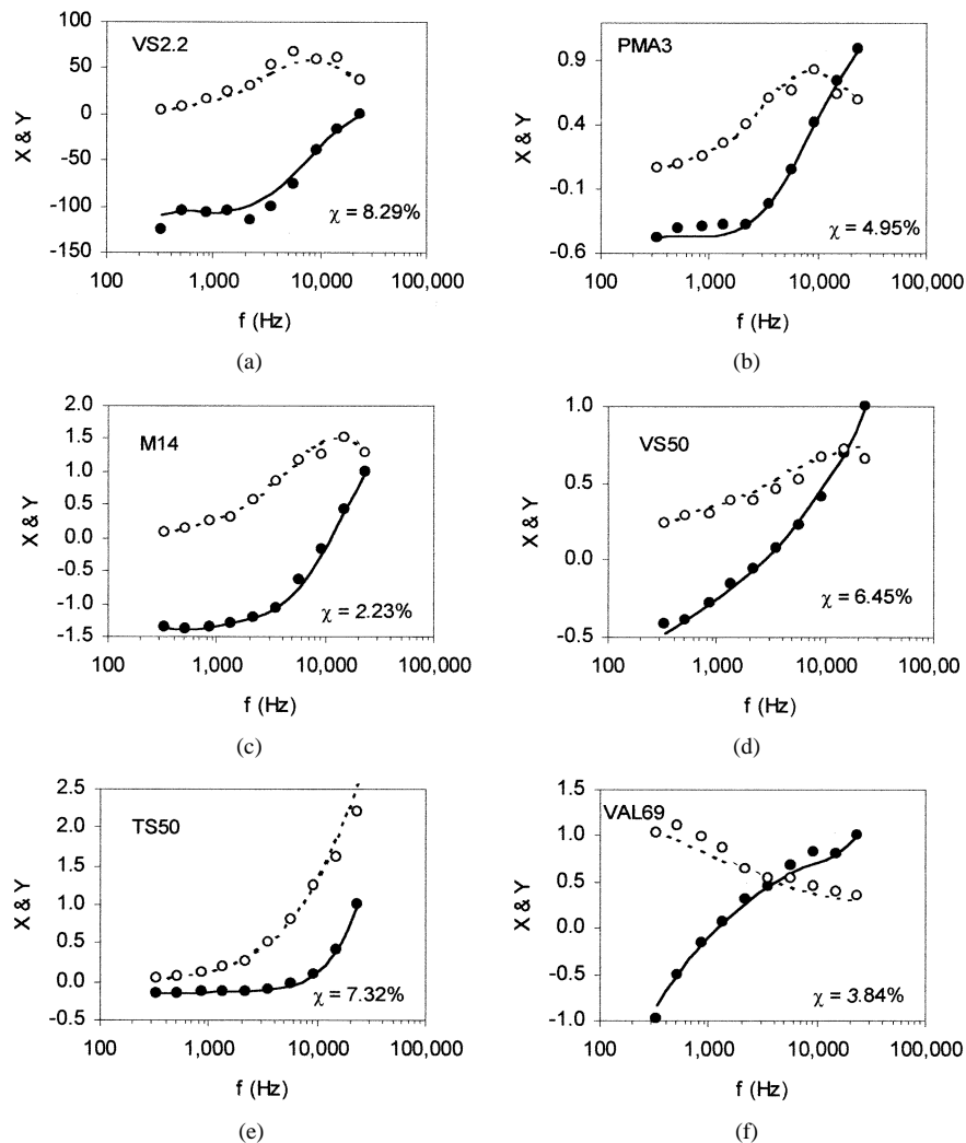
Fig. 8. Measured EMIS spectra (circles) obtained from six landmines, along with the best matching library landmine spectra (lines) all of which are correctly identified.
