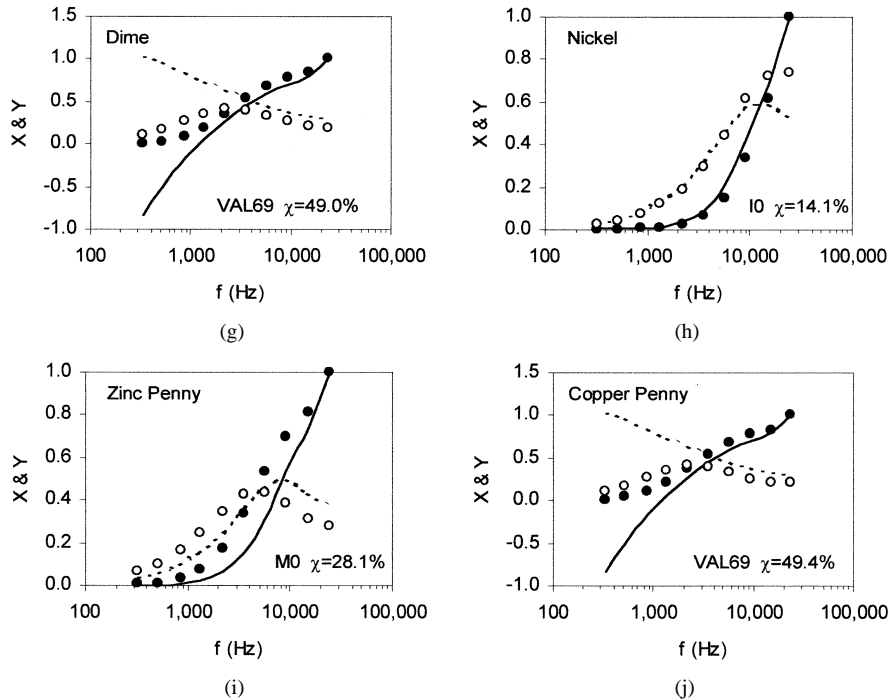
Fig. 9. (Continued) Normalized spectra of selected clutter items (circles), along with the best matching library spectra (lines) shown in Figs. 7 and 8. It is obvious that majority of the clutter can be correctly rejected.
