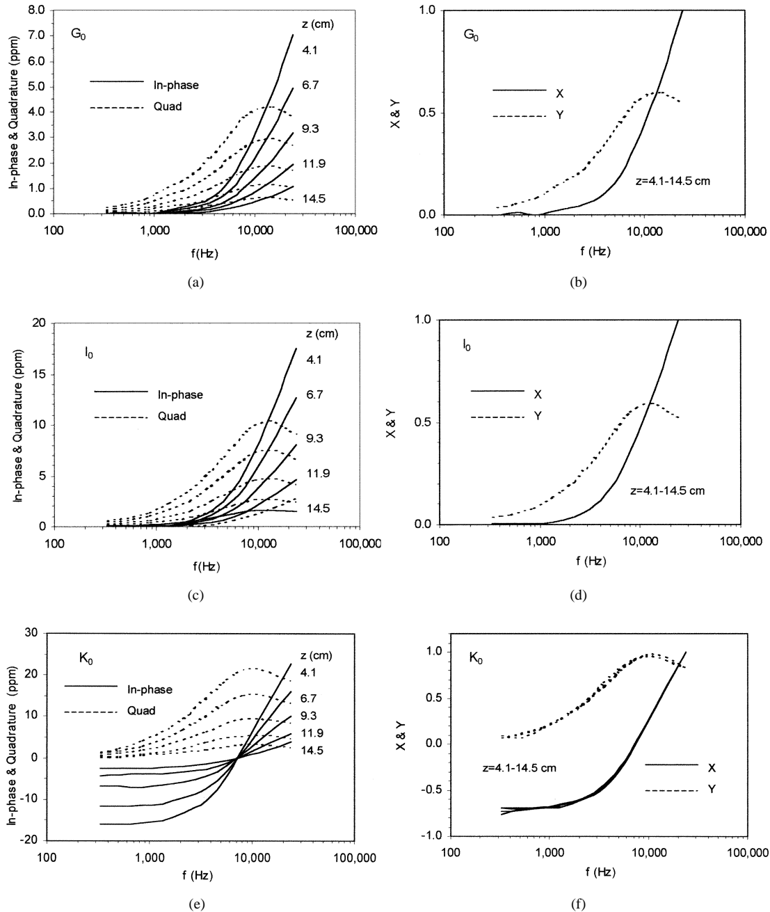
Fig. 6. Measured EMIS spectra (left) for five mine simulants G_0 , I_0 , K_0 , M_0 , and O_0 located at varying distances to the GEM-3 sensor and their corresponding normalized EMIS spectra (right).
