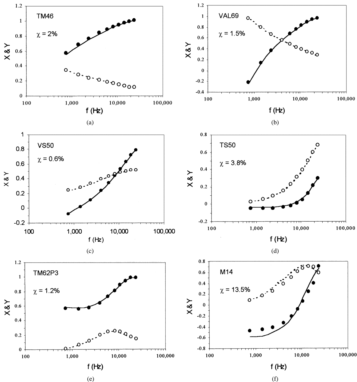
Fig. 10. Normalized EMIS spectra (circles) obtained from six blind grids at U.S. Army Test Site, along with the best matching library landmine spectra (lines). Each target was declared as the indicated best matching landmine.
