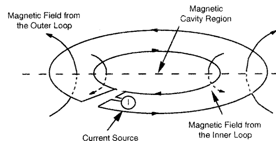
Fig. 2. Conceptual representation of creating a central magnetic cavity region using two concentric, circular loops that are electrically connected in an opposing polarity.
