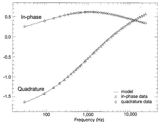
Fig. 3. GEM-3 data from a three-inch diameter chrome steel sphere compared to the sphere model (measured in air at a height of 37.3 cm).
