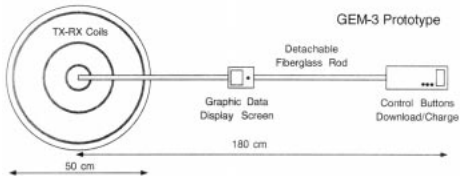
Fig. 1. Top: photograph of the GEM-3 monostatic broadband EMI sensor. Bottom: schematic diagram showing its internal construction.
