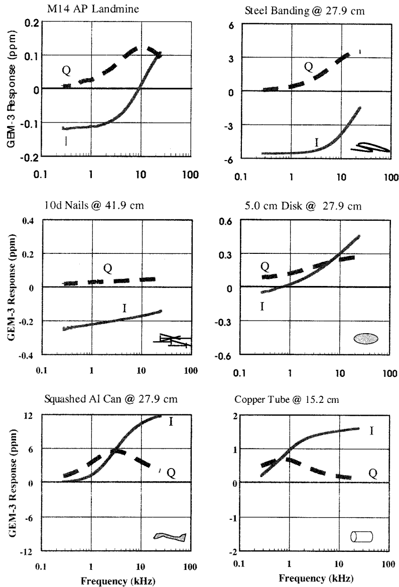
Fig. 6. EMIS spectra measured by the GEM-3 for an M-14 plastic landmine compared with various ordinary clutter items. We note that the EMIS spectrum of the M-14 is clearly distinguishable from the clutter and thus can greatly reduce the false alarm rate, which, in turn, would reduce the cost of clearing a minefield.
