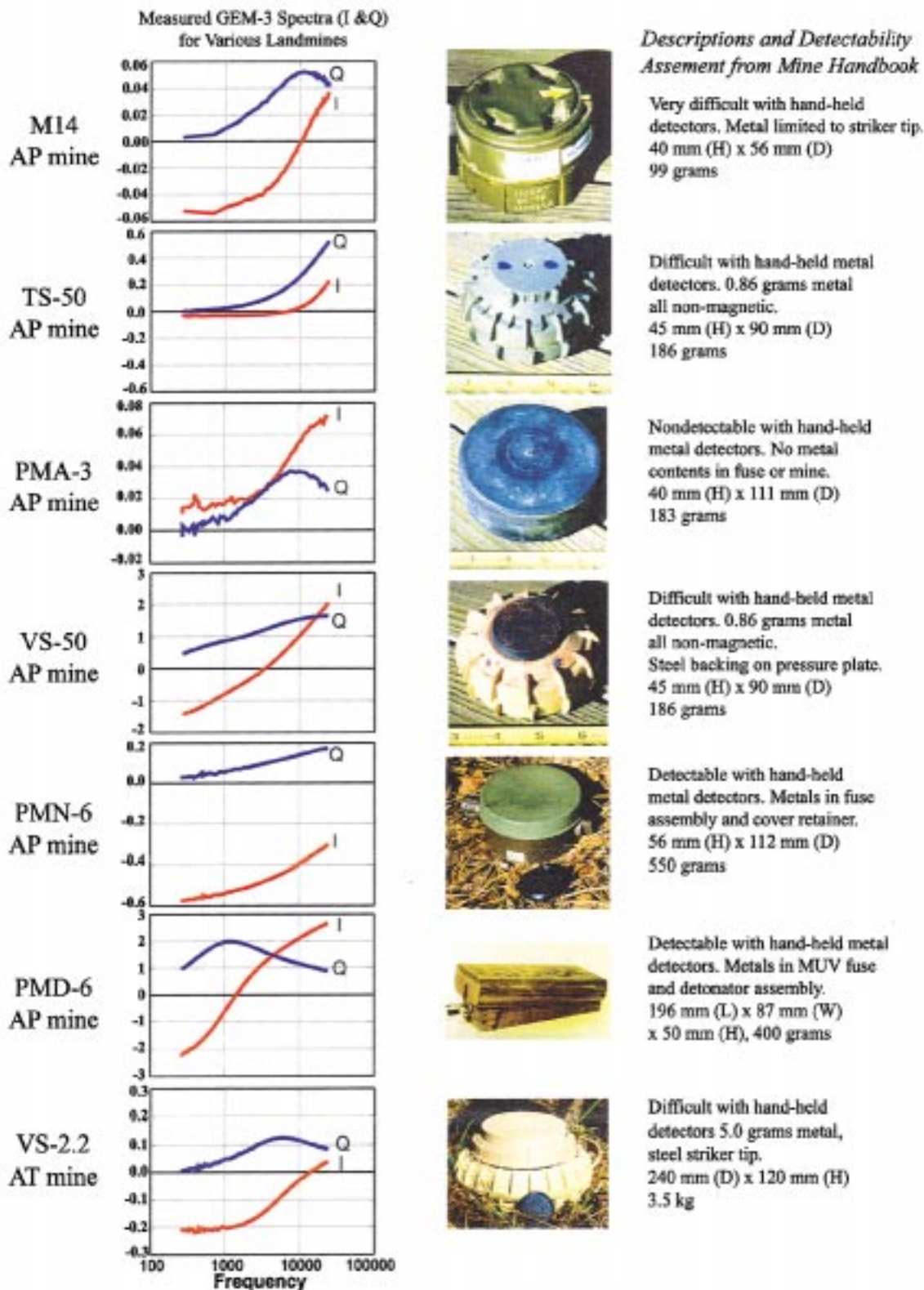
Fig. 5. EMIS spectra measured by the GEM-3 for various landmines, along with their photographs. Shown on the right is the commentary on the construction and detectability of each mine. The vertical axis has a ppm unit as defined in the text. M-14 and PMA-3 are common plastic mines that have very small metal parts, showing amplitudes less than 0.1 ppm. We note that each mine has a clearly detectable and distinct EMIS spectrum.
