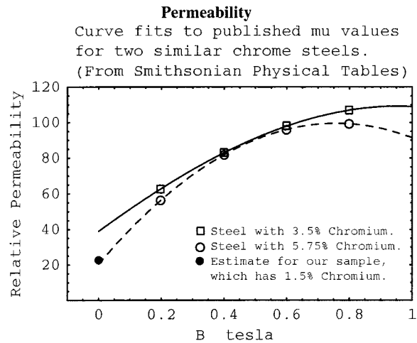
Fig. 4. Comparison between model fits of conductivity and permeability to published values for similar metals.
